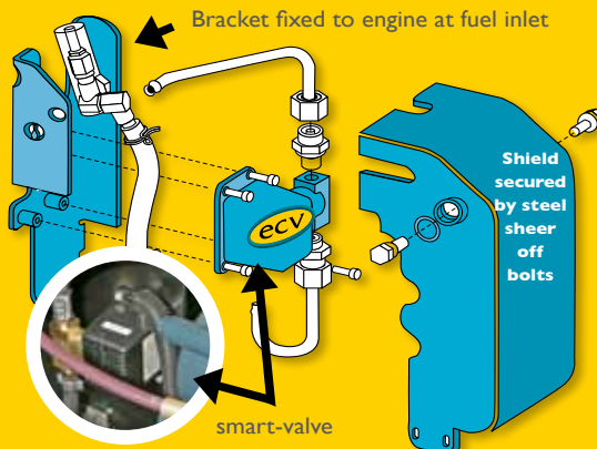
ECV - Electronic Coded Valve on Takeuchi at Intermat 2009
